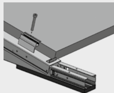
solar panel (provided by installer)
